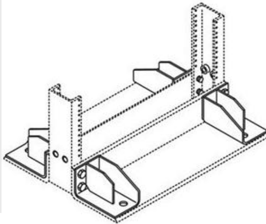
Fabrication Assy.
